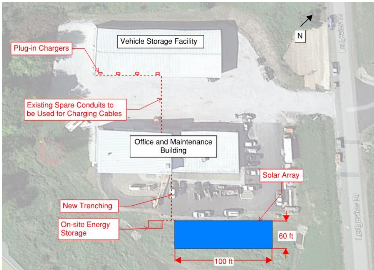
Figure 8 Conceptual Layout
